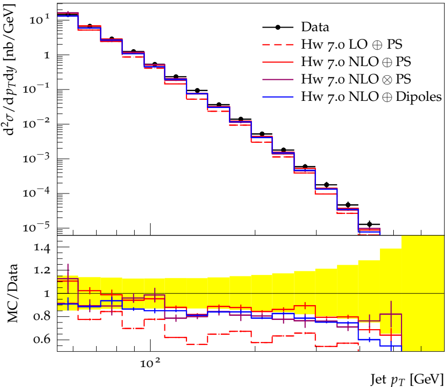
Inclusive jet cross-section vs p_T for |\eta| < 0.1, D = 0.7
