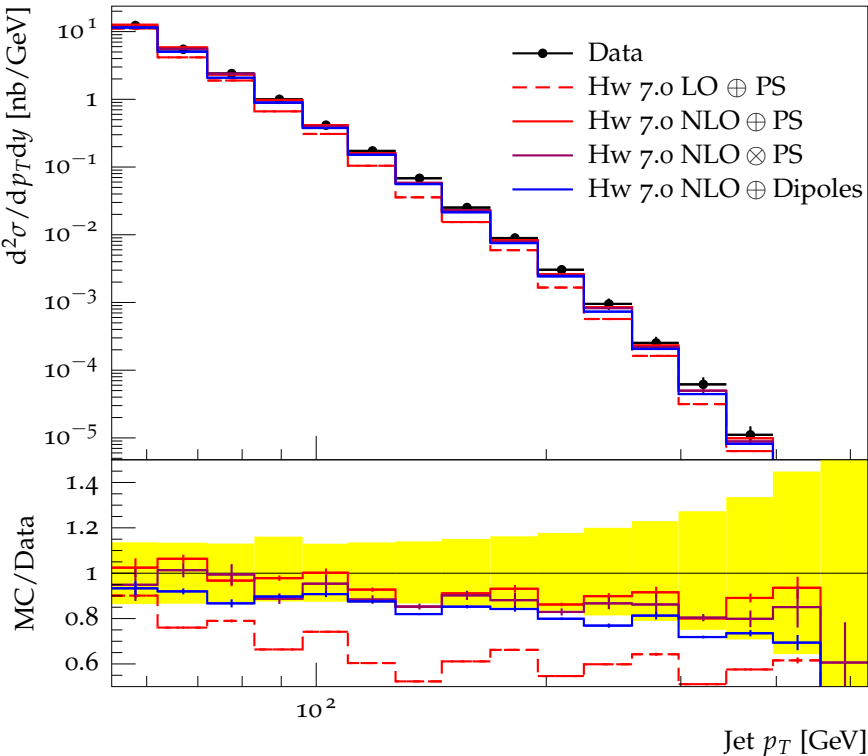
Inclusive jet cross-section vs p_T for 0.7 < |\eta| < 1.1, D = 0.7
