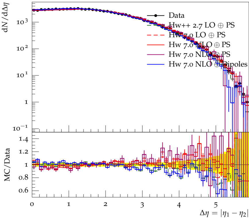
Pseudorapidity difference of the two opposite jets
