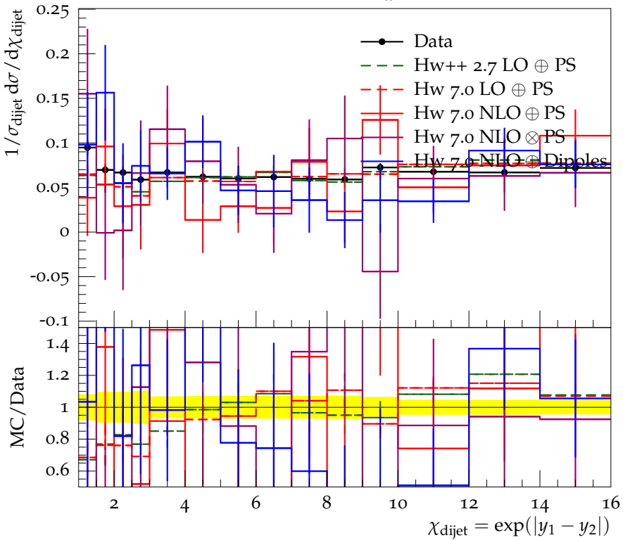
Dijet angular distribution in 0.5 < M_{jj}/\text{TeV} < 0.6
