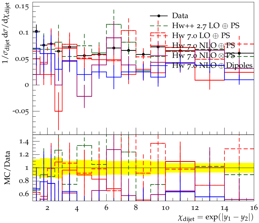
Dijet angular distribution in 0.8 < M_{jj}/\text{TeV} < 0.9
