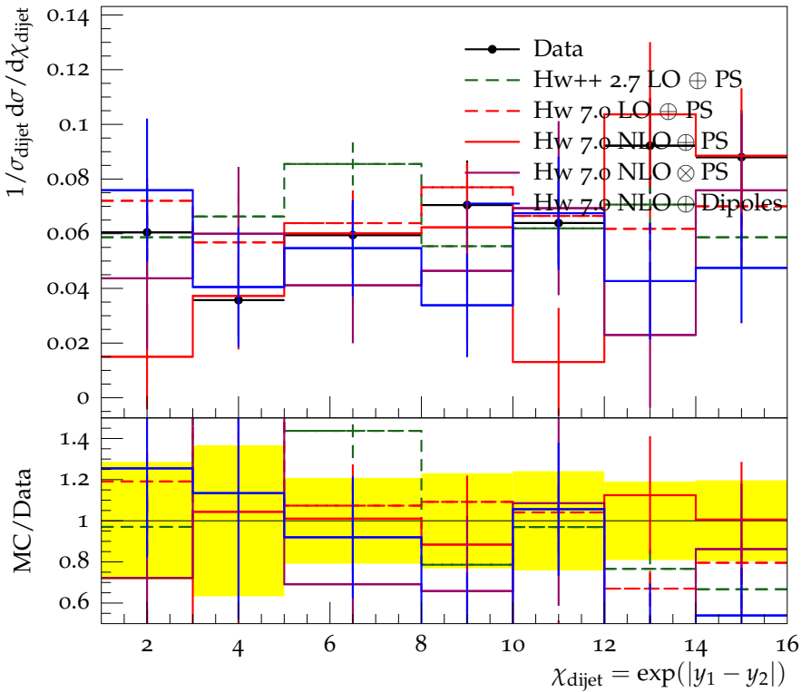
Dijet angular distribution in 1.0 < M_{jj}/\text{TeV} < 1.1
