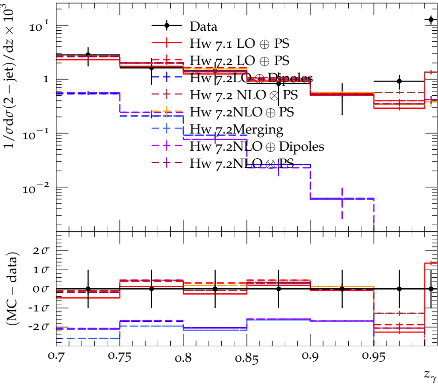
Photon Fragmentation in 2-jet events with y_{\text{cut}} = 0.06
