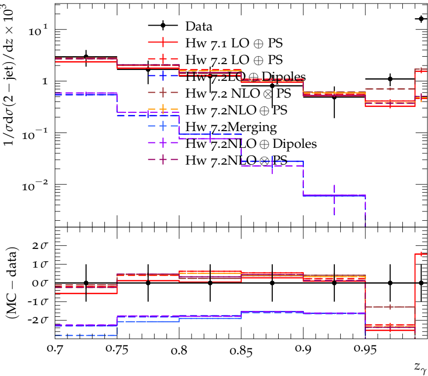
Photon Fragmentation in 2-jet events with y_{\text{cut}} = 0.1
