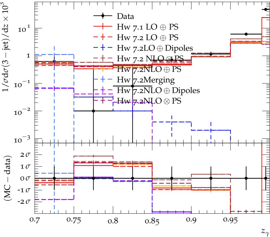
Photon Fragmentation in 3-jet events with y_{\text{cut}} = 0.06
