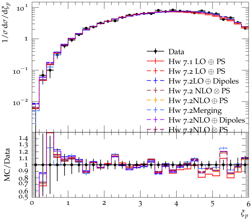
Charged particle spectrum ( E_{\text{CMS}} = 161 \text{ GeV} )
