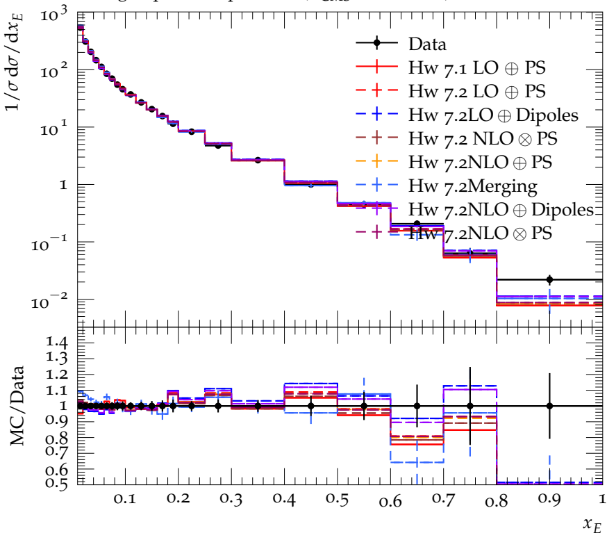
Charged particle spectrum ( E_{\text{CMS}} = 189 \text{ GeV} )
