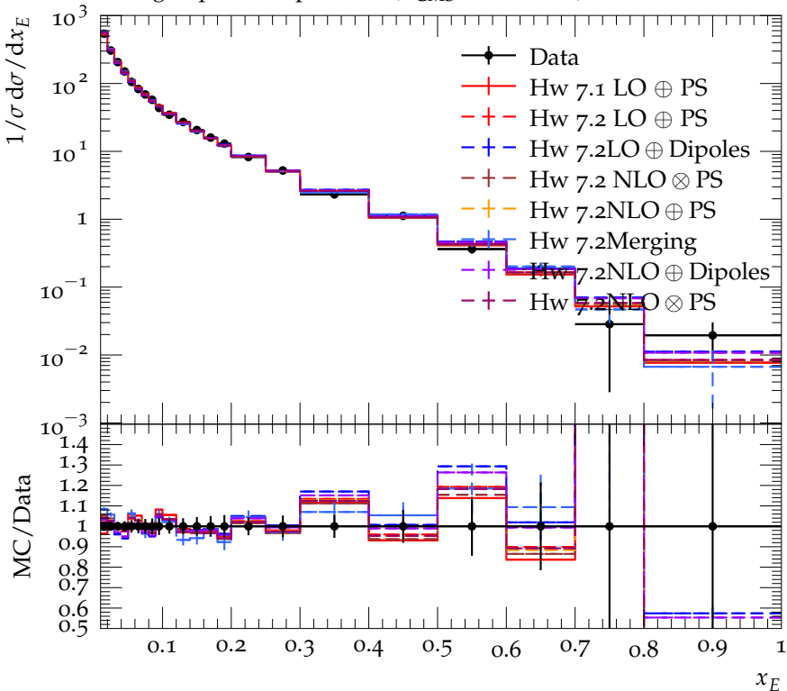
Charged particle spectrum ( E_{\text{CMS}} = 200 \text{ GeV} )
