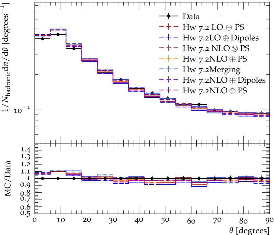
Charged particle flow w.r.t the sphericity axis
