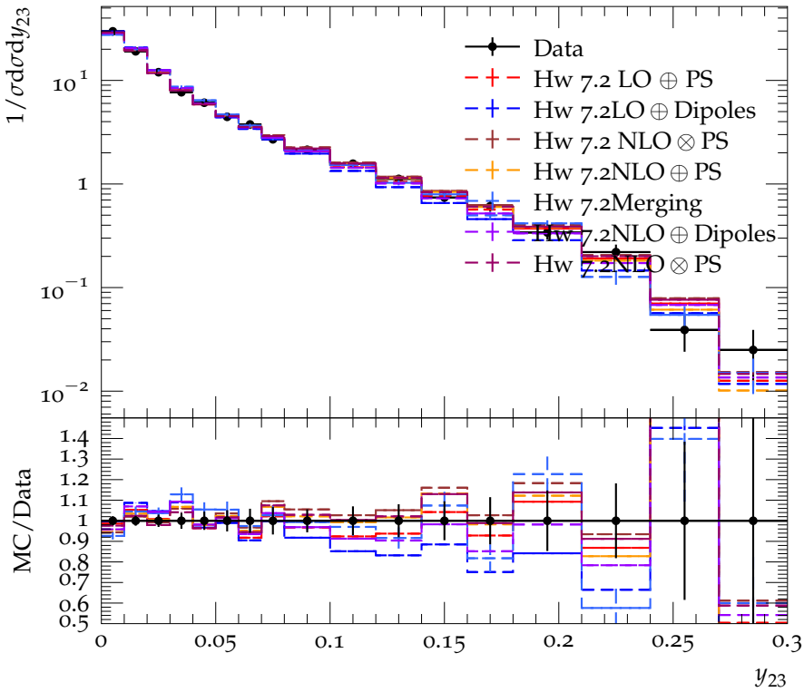
y_{23} in the JADE algorithm (p-scheme)
