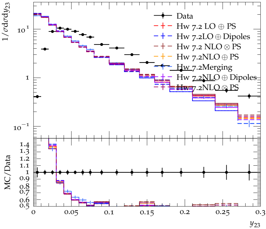
y_{23} in the JADE algorithm (E-scheme)
