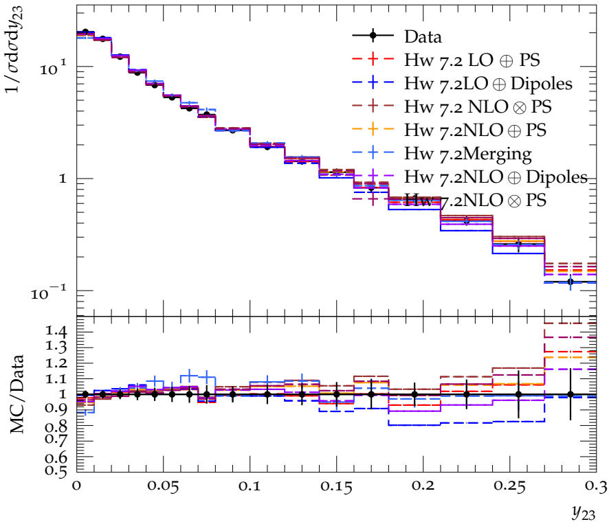
y_{23} in the JADE algorithm (Eo-scheme)
