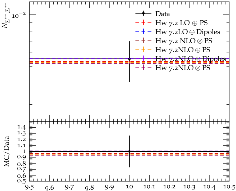
Multiplicity of \Sigma^{*-} , \bar{\Sigma}^{*+} in the continuum (10 GeV)
