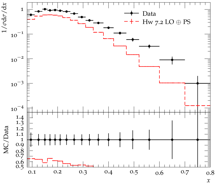
Spectrum of \Lambda^0, \bar{\Lambda}^0 in Y(1S) decays
