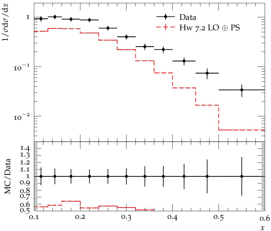
Spectrum of \Lambda^0, \bar{\Lambda}^0 in Y(2S) decays
