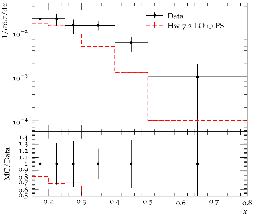
Spectrum of \Xi^- , \bar{\Xi}^- in Y(2S) decays
