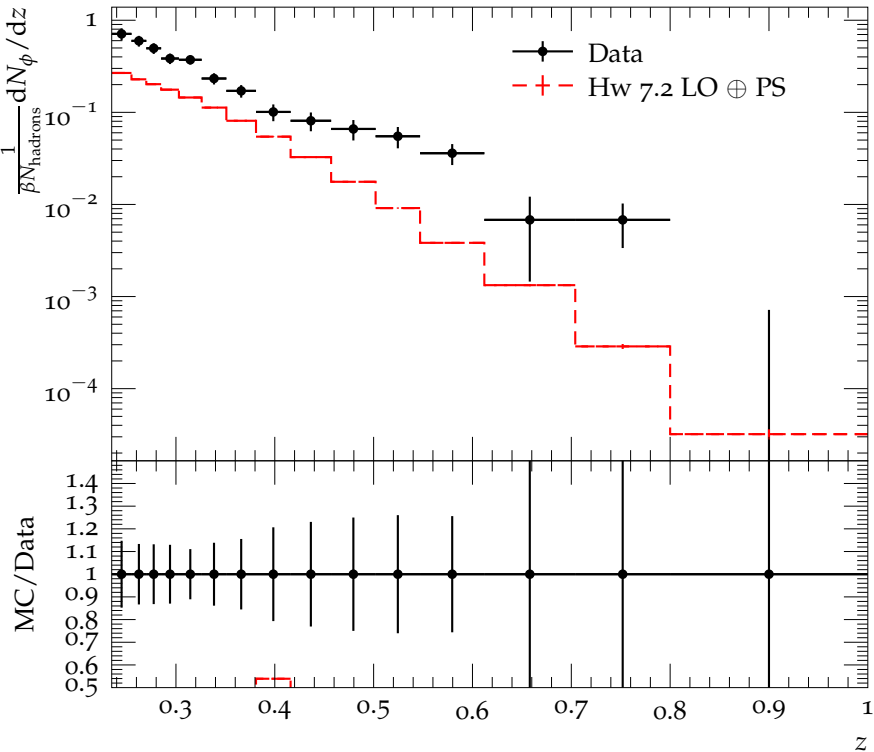
\phi spectrum in Y(1S) decays
