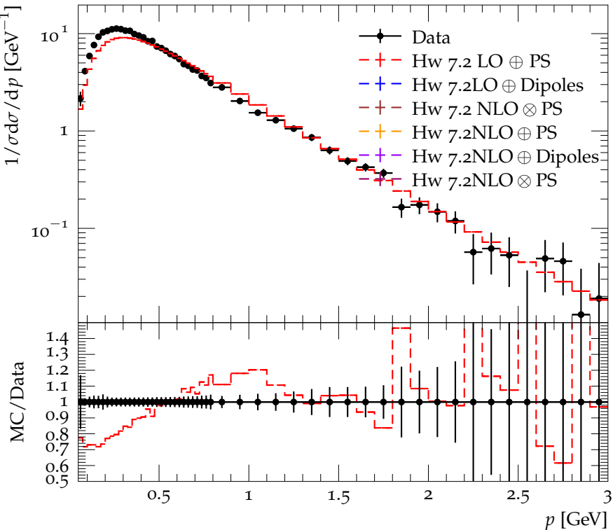
Spectrum of \pi^\pm in Y(1S) decays
