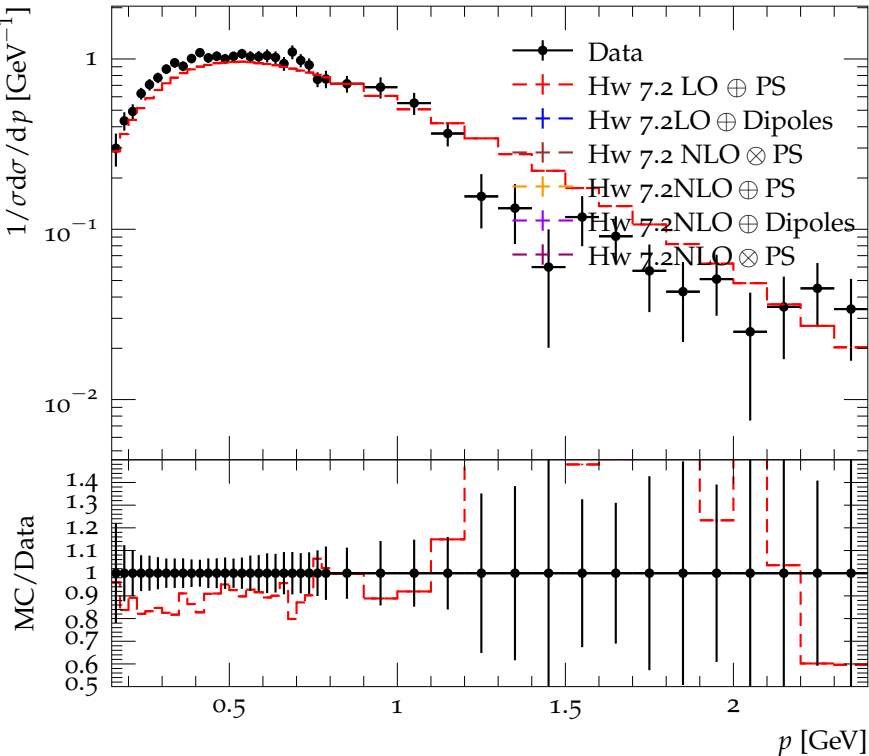
Spectrum of K^\pm in Y(1S) decays
