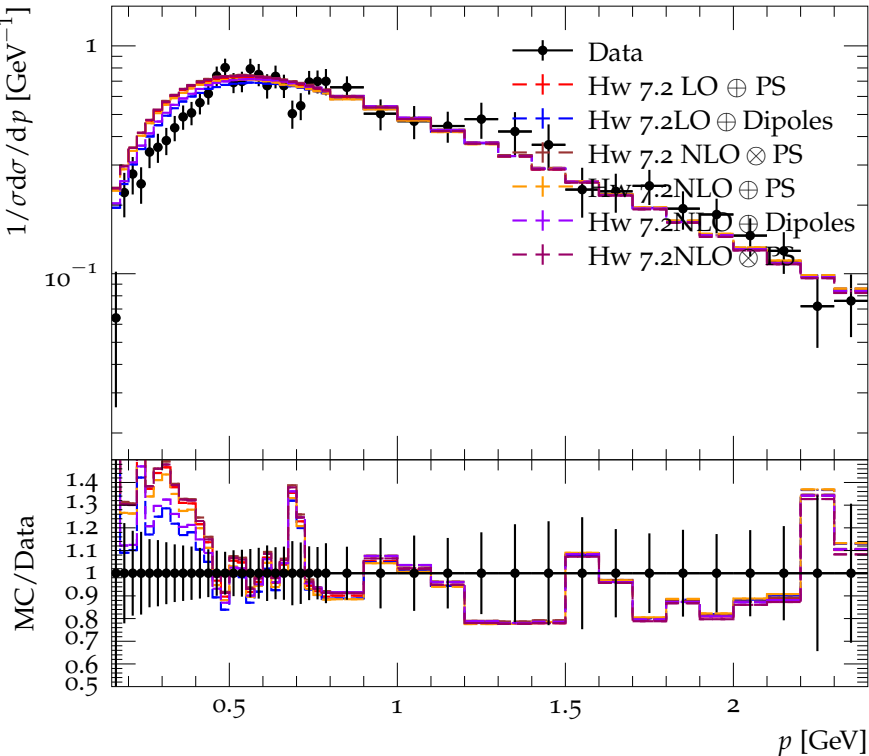
Spectrum of K^\pm in continuum (10 GeV)
