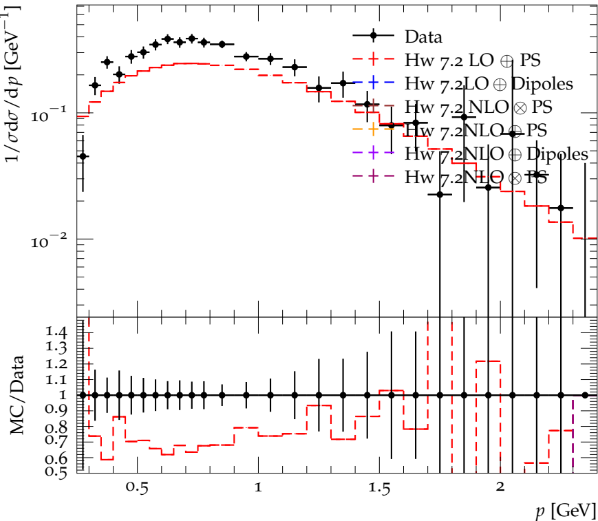
Spectrum of p, \bar{p} in Y(1S) decays
