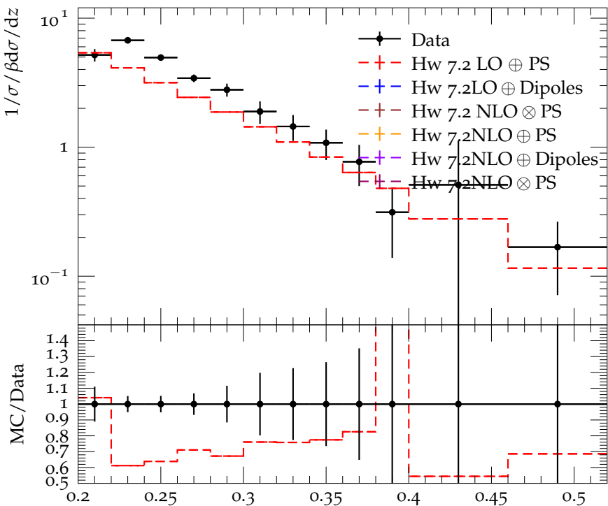
Spectrum of p, \bar{p} in Y(1S) decays
