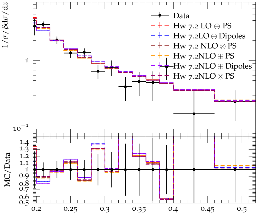
Spectrum of p, \bar{p} in continuum (10 GeV)
