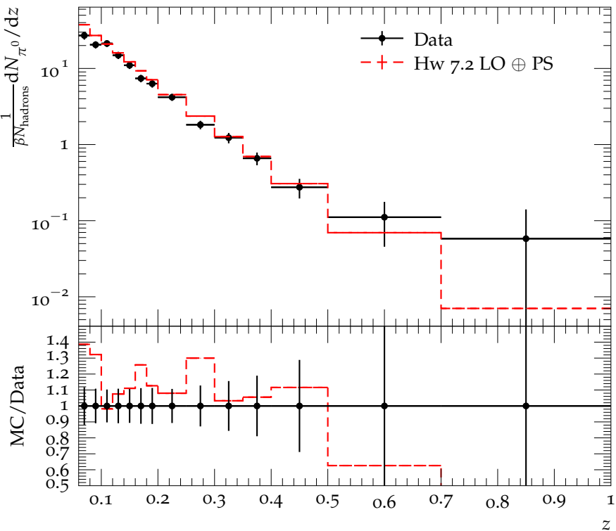
\pi^0 spectrum in Y(2S) decays
