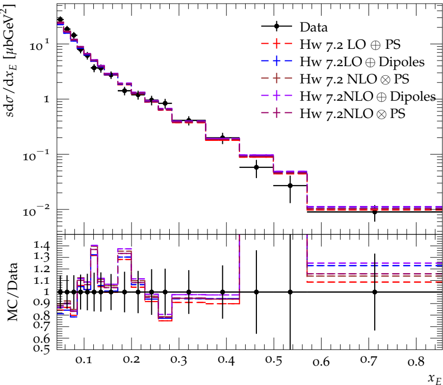
Photon spectrum at E_{\text{CMS}} = 14 \text{ GeV}
