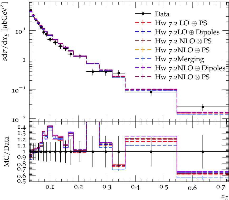
Photon spectrum at E_{\text{CMS}} = 22 \text{ GeV}
