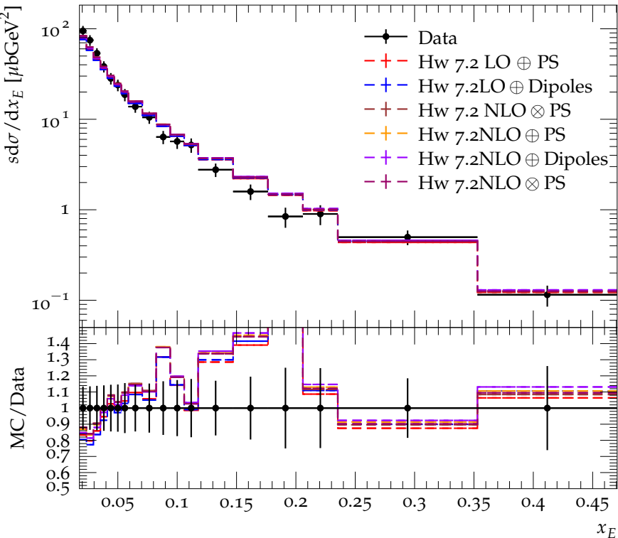
Photon spectrum at E_{\text{CMS}} = 34 \text{ GeV}
