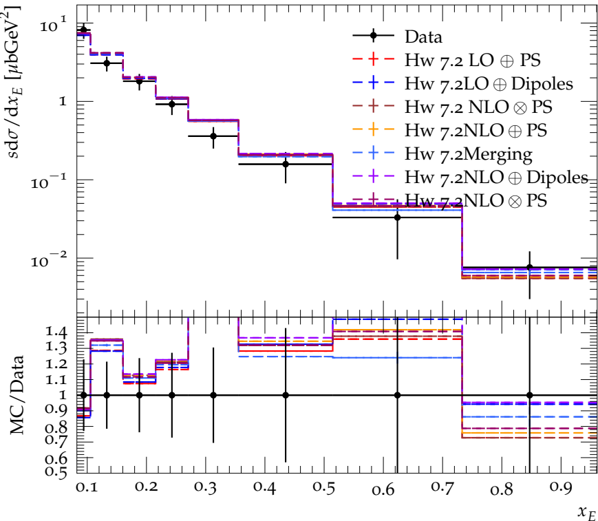
\pi^0 spectrum at E_{\text{CMS}} = 22 GeV
