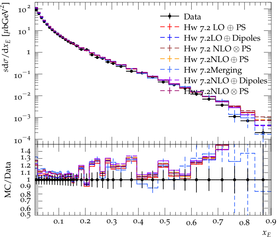
Photon spectrum at E_{\text{CMS}} = 35 GeV
