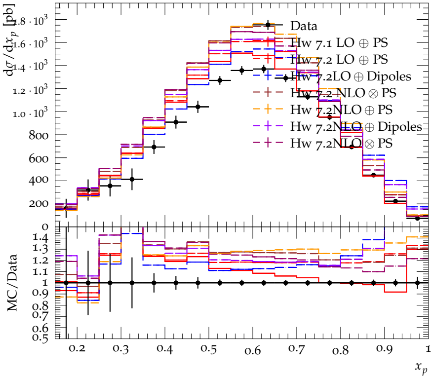
Average D meson scaled momentum distribution
