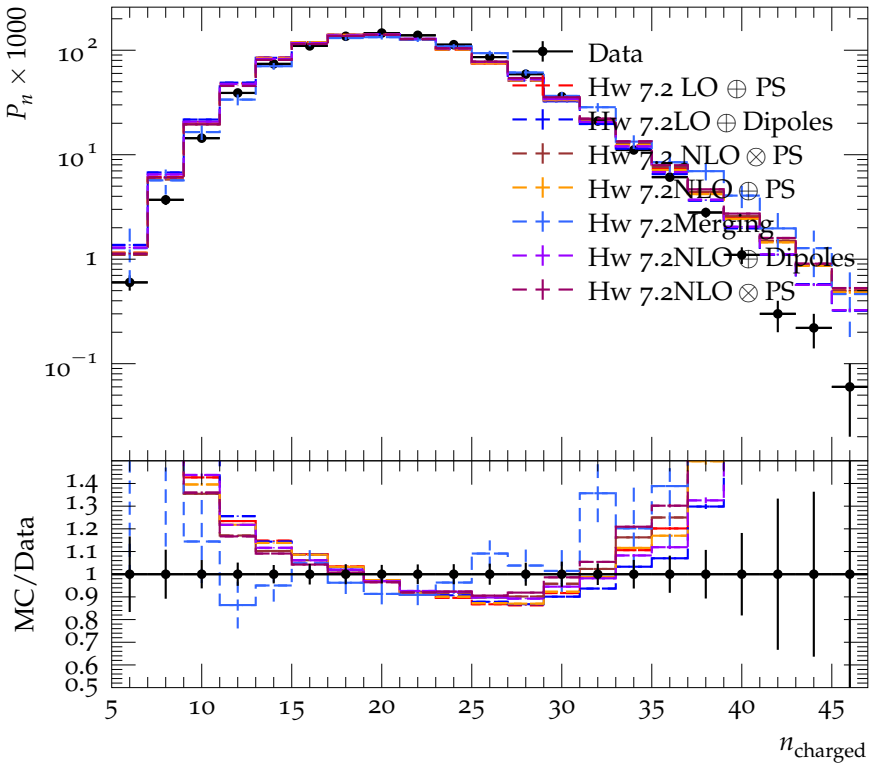
Charged parton multiplicity, 3-jets, y_{\text{cut}} = 0.01
