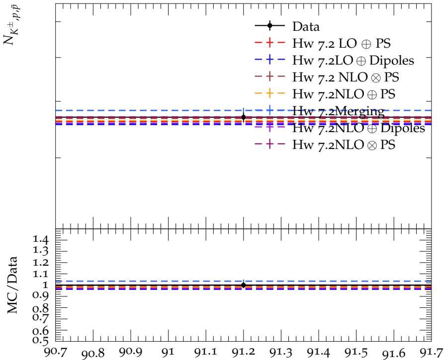
K^\pm, p, \bar{p} Multiplicity (bottom events)
