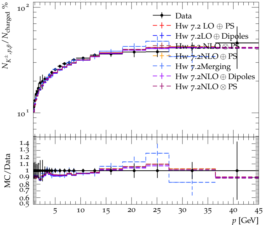
Ratio of N_{K^\pm, p, \bar{p}} to N_{\text{charged}} (all events)
