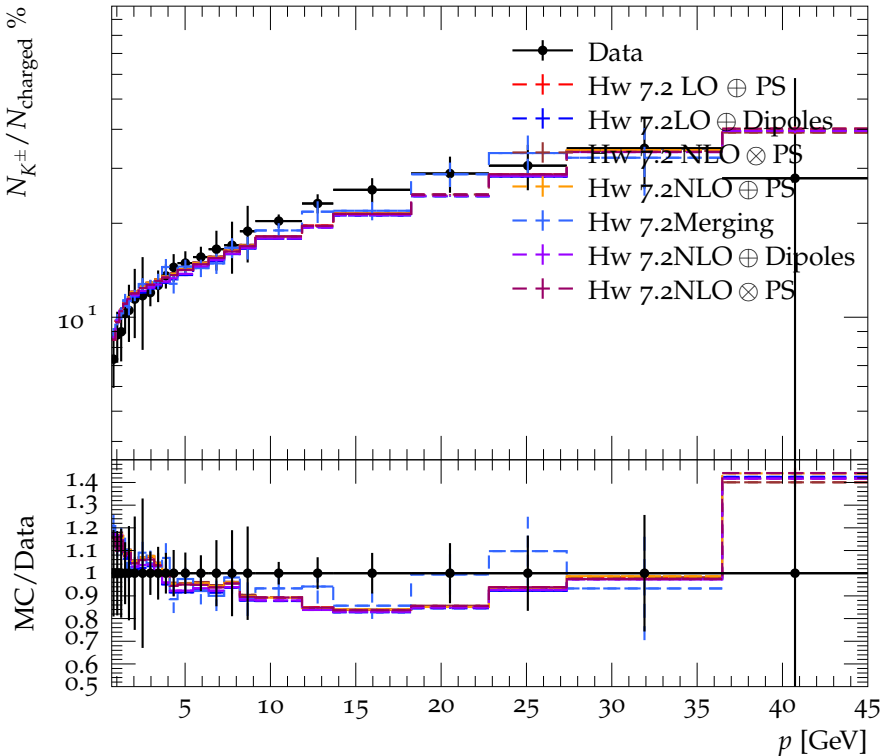
Ratio of N_{K^\pm} to N_{\text{charged}} (light events)
