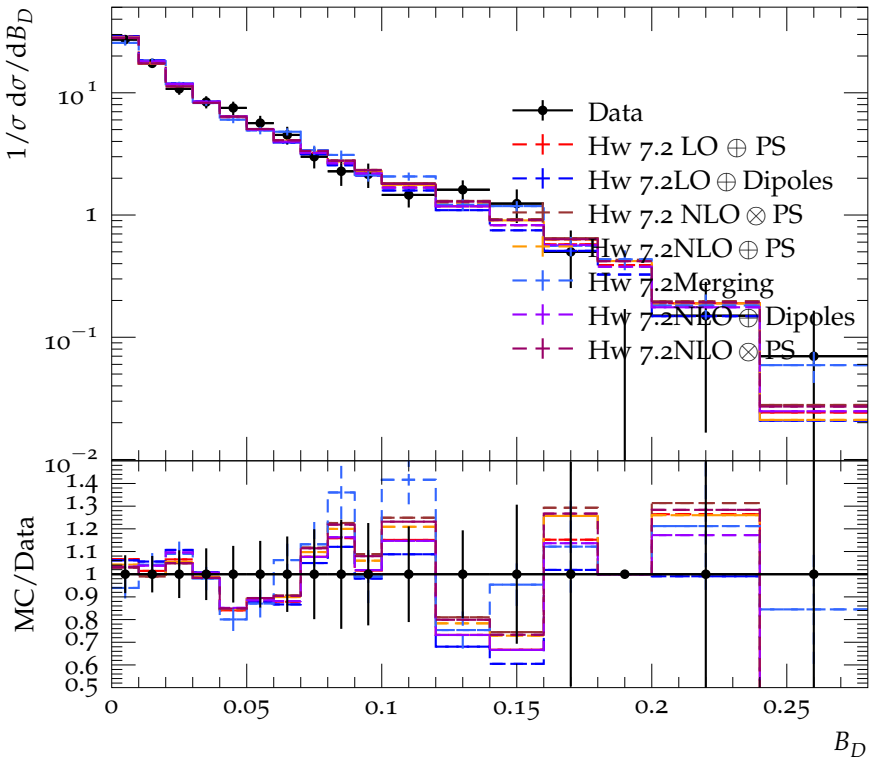
Difference of the jet broadenings ( E_{\text{CMS}} = 183 \text{ GeV} )
