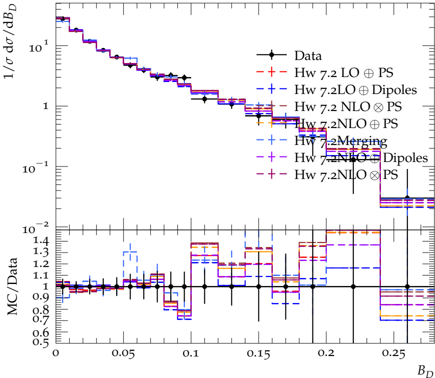
Difference of the jet broadenings ( E_{\text{CMS}} = 189 \text{ GeV} )
