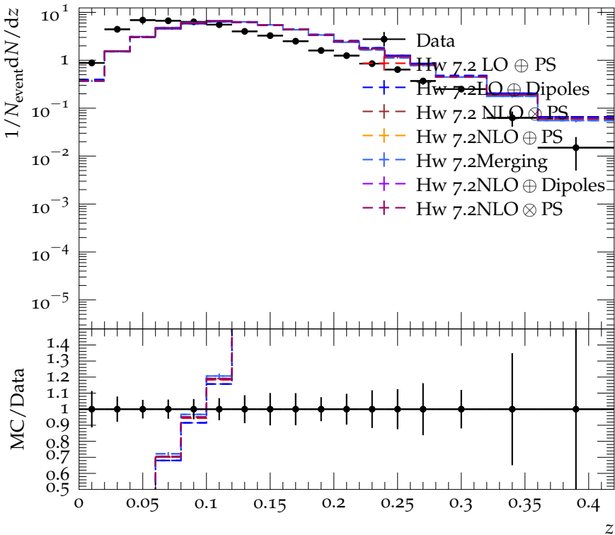
Momentum Fraction of 2nd Highest z particle (2 jet sample)
