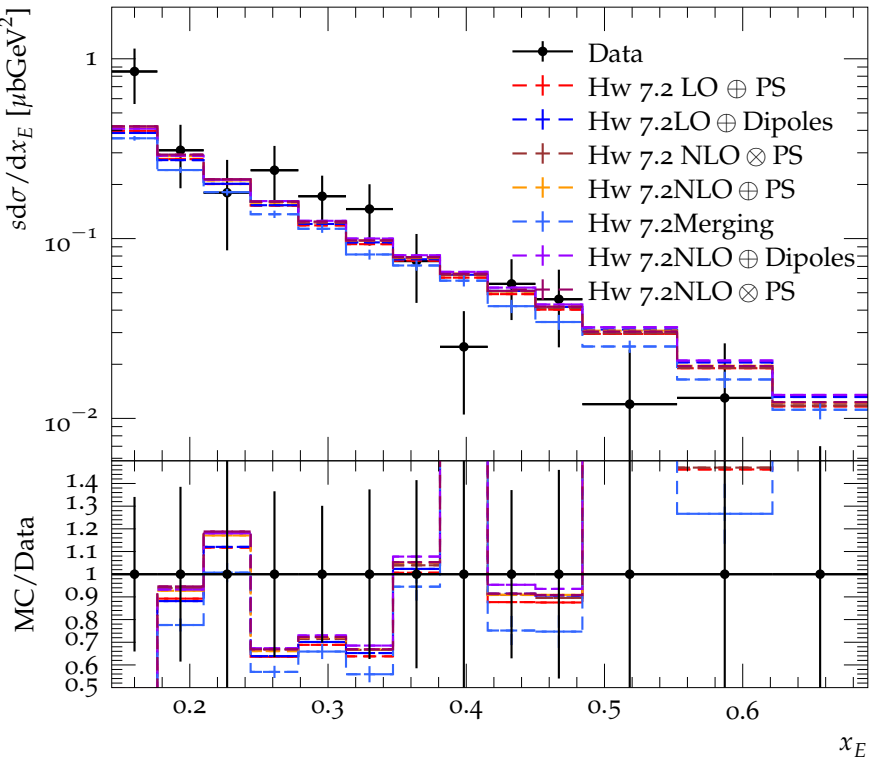
\eta spectrum at E_{\text{CMS}} = 29 GeV
