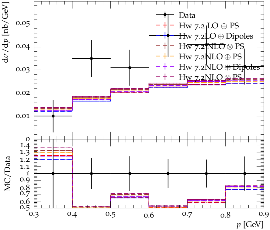
\bar{p} spectrum at 34 GeV
