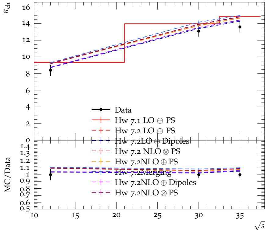
Mean charged multiplicity average for \sqrt{s} between 12 and 35 GeV
