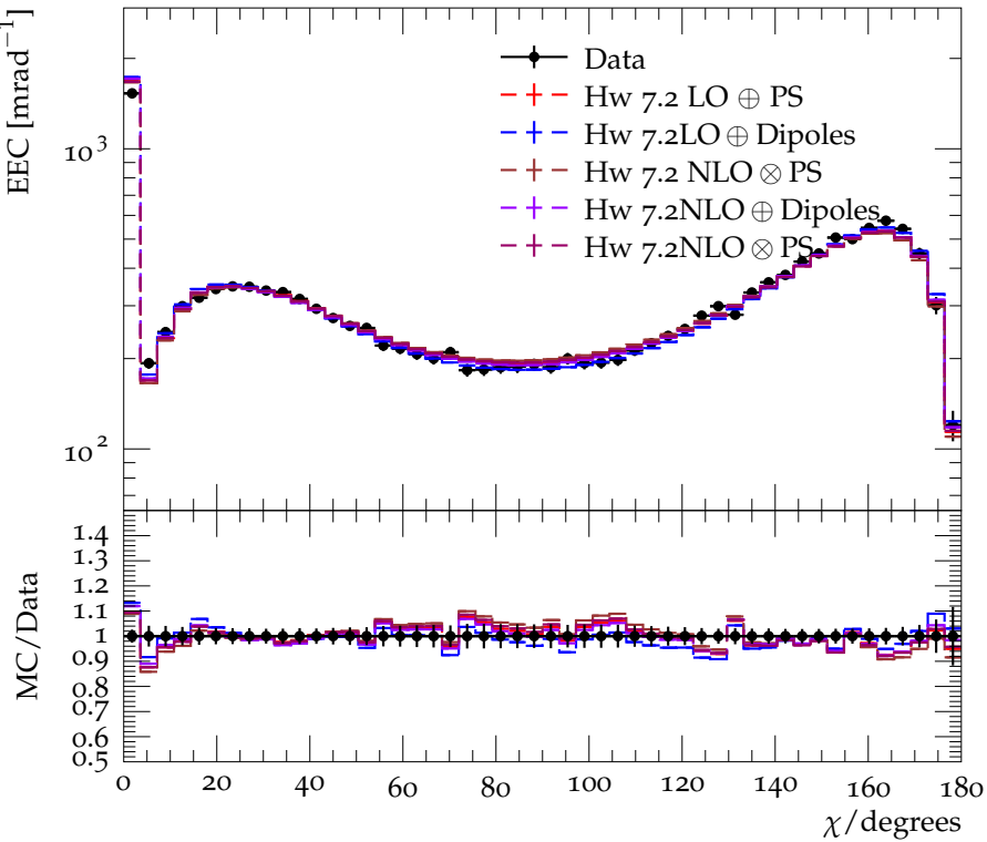
Energy-energy correlation at E_{\text{CMS}} = 14 GeV
