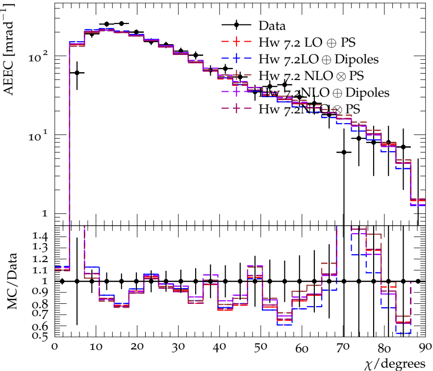
Asymmetry of the energy-energy correlation at E_{\text{CMS}} = 14 GeV
