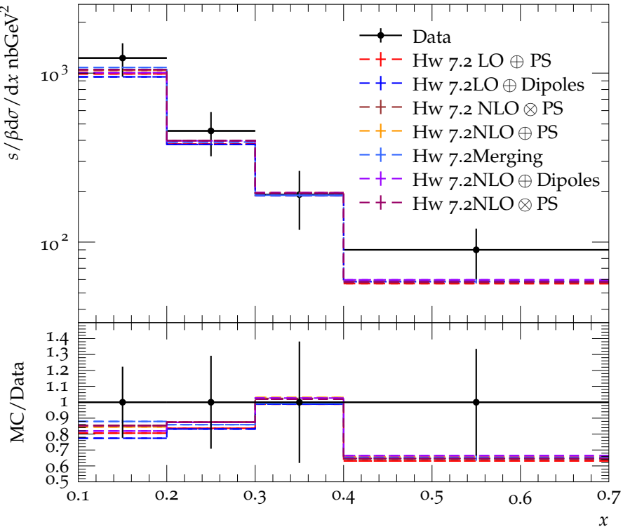
\rho^0 scaled momentum spectrum for E_{\text{CMS}} = 35 GeV
