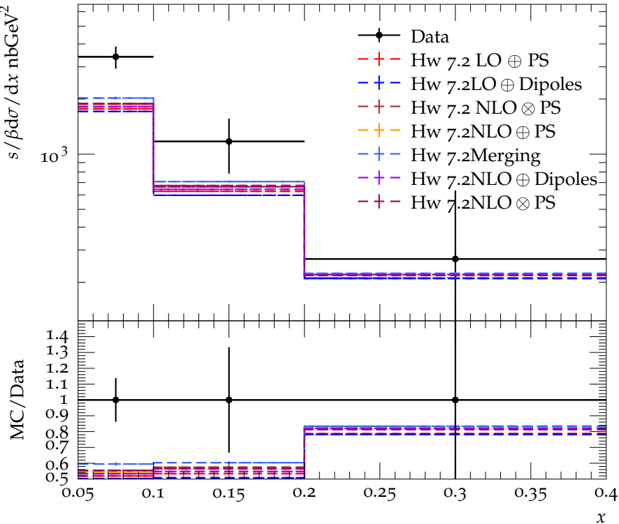
K^{*\pm} scaled momentum spectrum for E_{\text{CMS}} = 35 GeV
