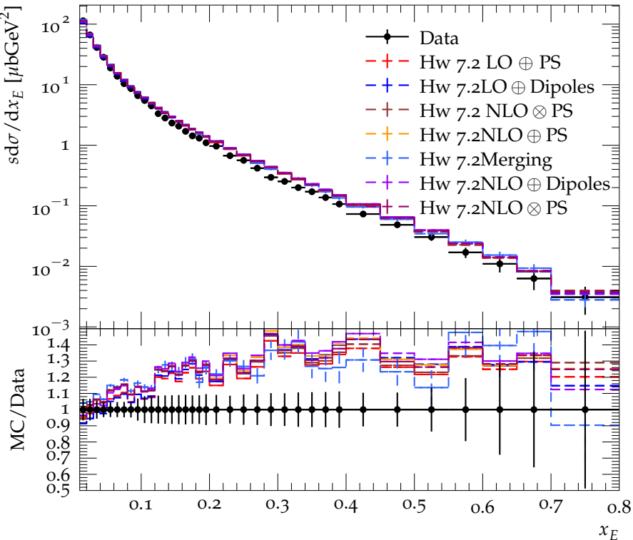
\gamma scaled energy spectrum at 35 GeV
