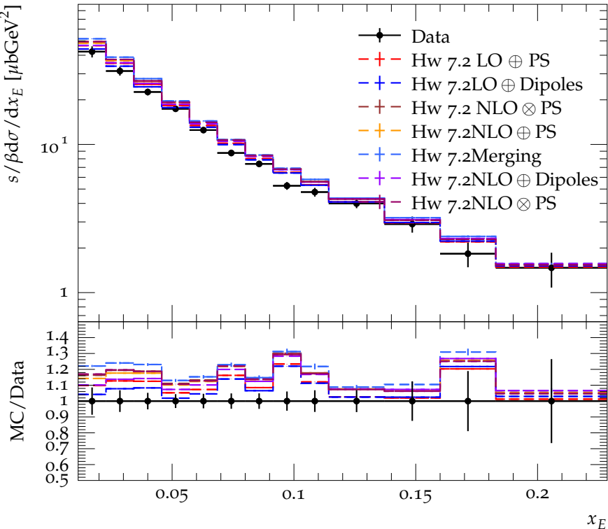
\pi^0 scaled energy spectrum at 35 GeV
